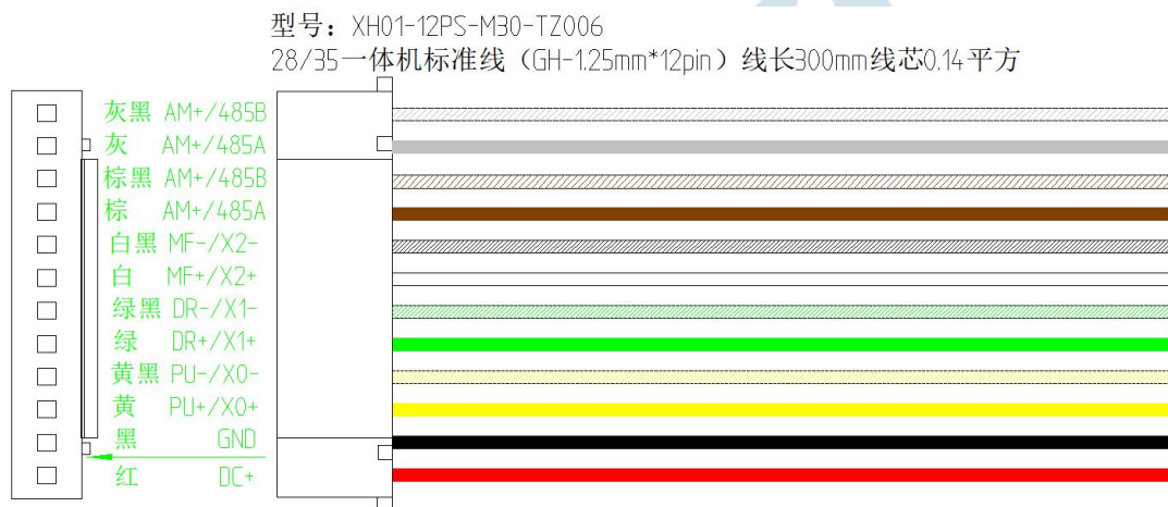
Figure 6.2IDH28Series wiring diagram
