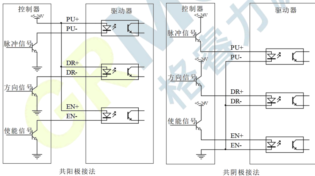
Figure 3.2 Input interface circuit
