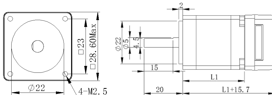
Figure 6.1 IDH28 Schematic diagram of the appearance of the series of integrated machines
